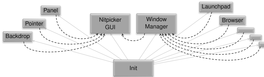
Figure 40: The nitpicker GUI accompanied with a window manager that interposes the nitpicker session interface for the applications on the right. The applications on the left are still able to use nitpicker directly and thereby avoid the complexity added by the window manager.
